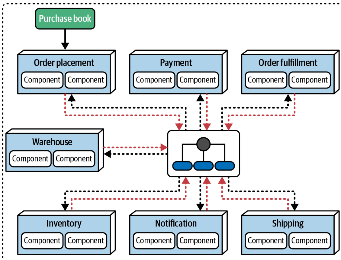
Figure 20-6. Using one broker for the entire workflow
