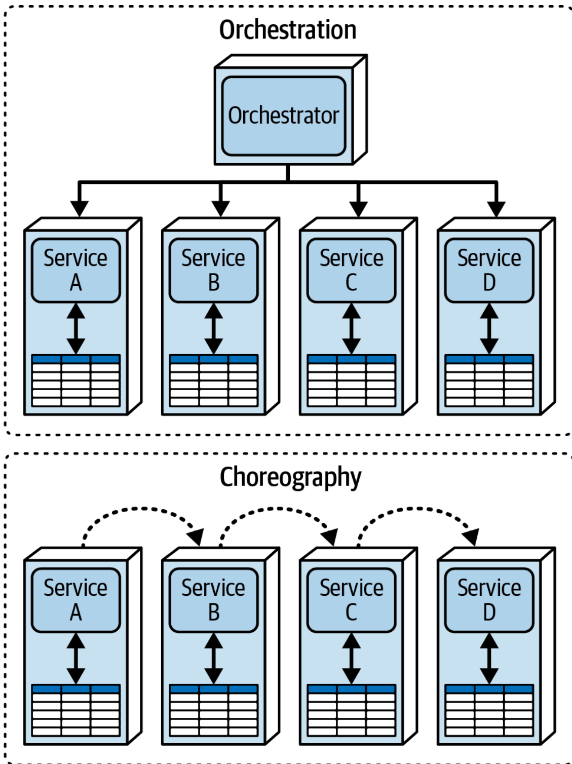
Figure 20-2. Orchestration and choreography in a microservices architecture
