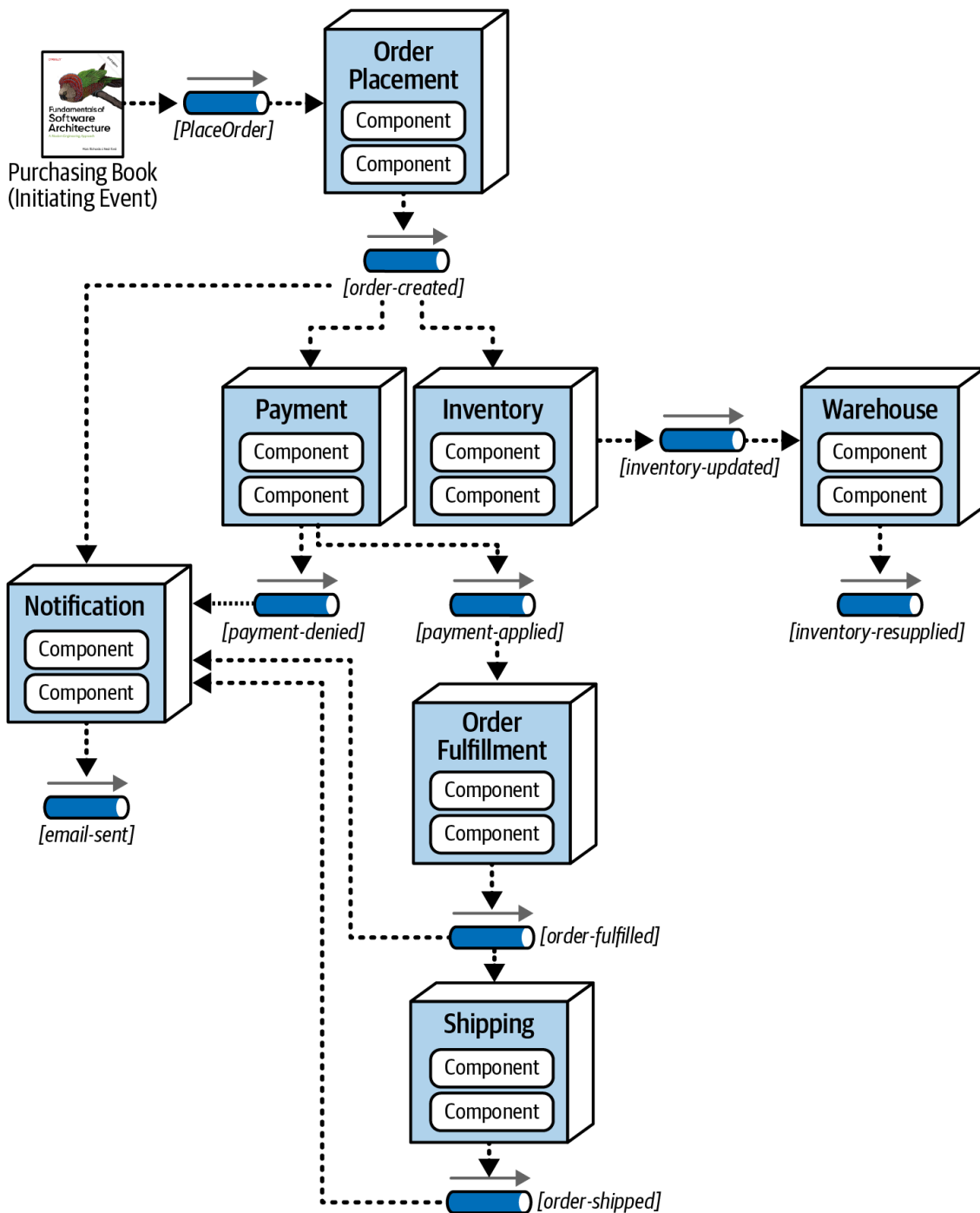
Figure 20-4. An order placement workflow implemented in EDA
