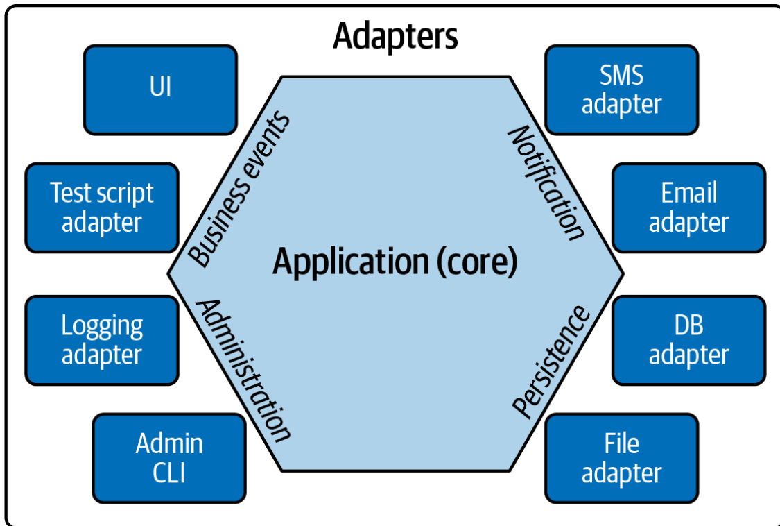
Figure 20-1. The Hexagonal architecture pattern
