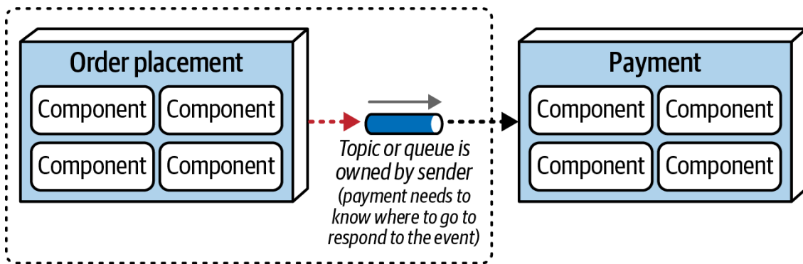
Figure 20-5. In event-driven choreography, the topic or queue is typically owned by the sender
