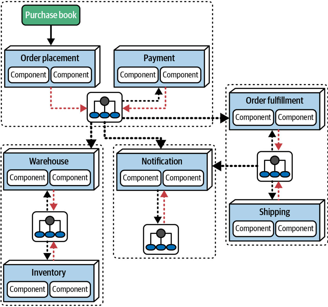
Figure 20-7. Utilizing the Domain-Broker pattern to assign ownership to infrastructure
