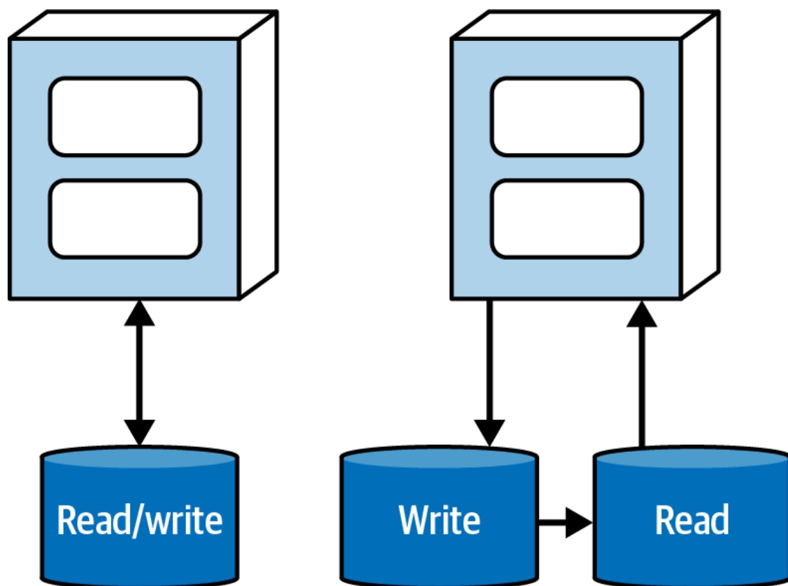
Figure 20-3. Client/server versus CQRS
